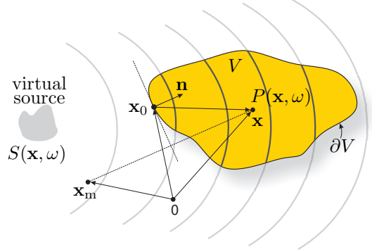
Figure 1: Geometrical parameters used for the Kirchhoff-Helmholtz integral (1) and monopole only reproduction.
