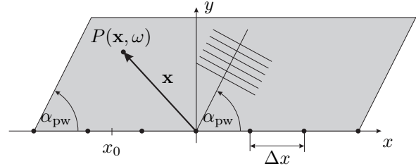
Figure 1: Geometry used to derive the sampling artifacts for linear loudspeaker arrays.
