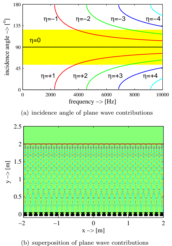
Figure 2: Reproduction of a bandlimited plane wave ( B = 10 kHz, \alpha_{\text{pw}} = 90^\circ ) on a linear WFS system ( \Delta x = 10 cm).
